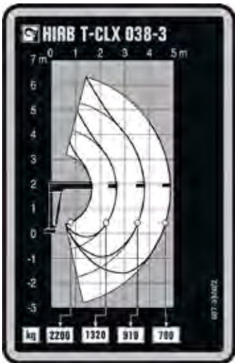
Load diagram HIAB T-CLX 038-3
